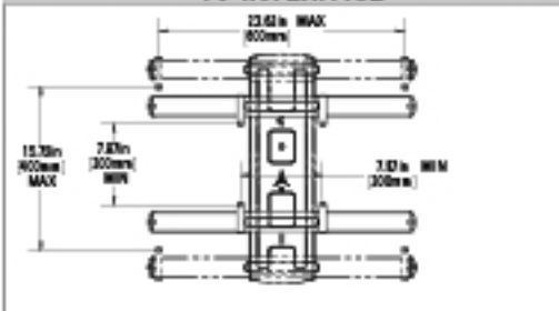
WALL PLATE
